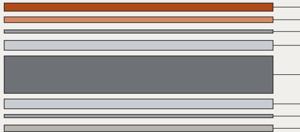
Pre-painted steel, top to bottom: topcoat, primer, pretreatment, metallic coating, steel, metallic coating, pretreatment, backcoat.
